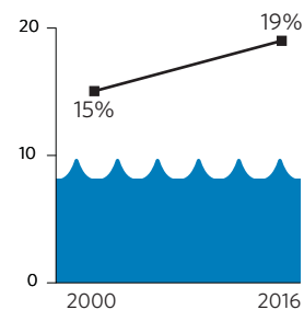
Proportion of marine key biodiversity areas under protection worldwide
